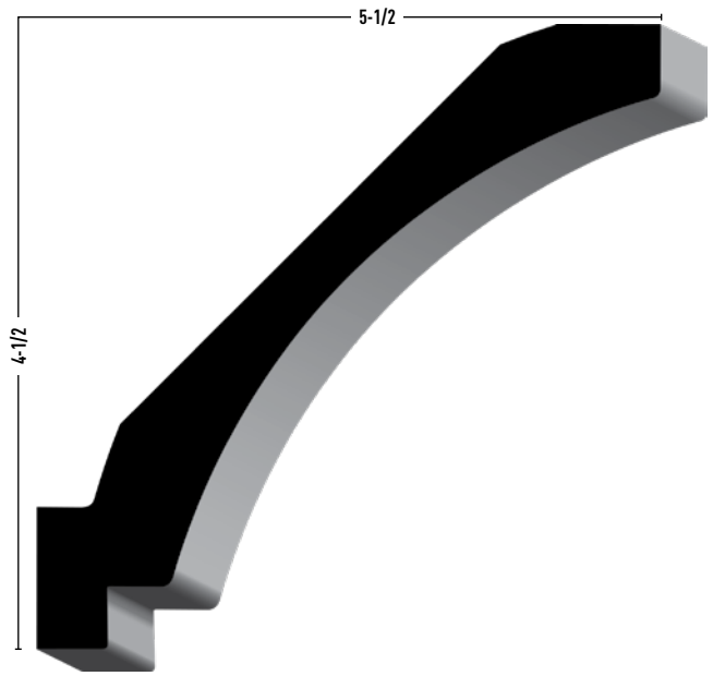
730 1-3/16 x 7 MDF 16'
