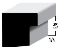
B G250 Eased Nose Back Band 1-1/16 x 1-1/16 PRIMED 16'
