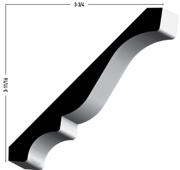
L 45 19/32 \times 5-1/4 MDF 16'
