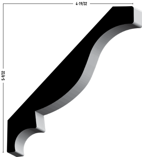
043 1 x 6-15/16 MDF 16'
