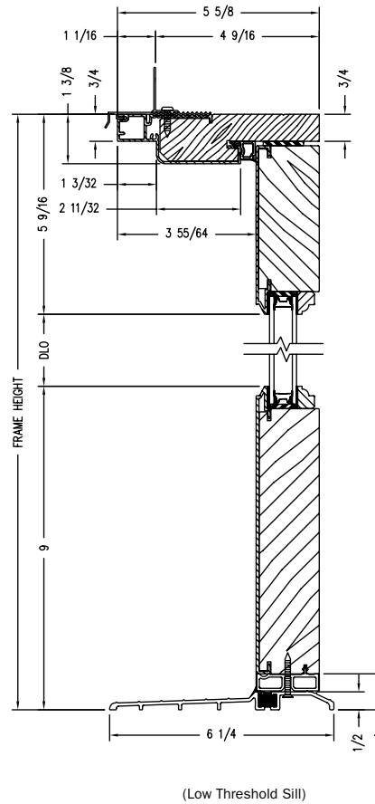
Vertical Section
